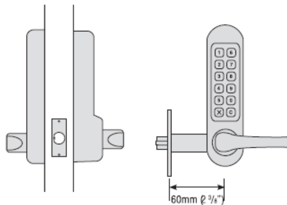
CL510/CL515 with tubular latchbolt
