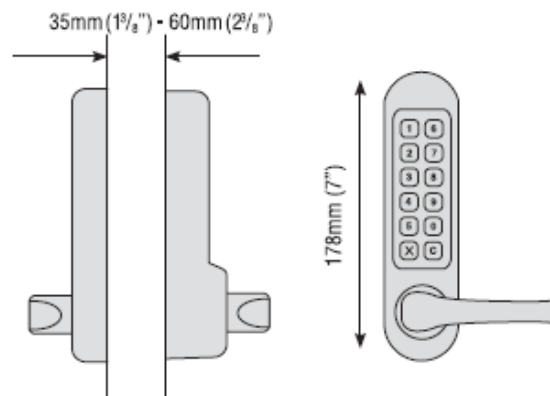
CL500/CL505 for use with existing lock
