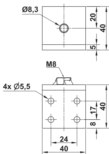
Bracket for the door part no. 205273 or 205274 (AISI 304)
