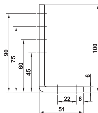
Angled bracket for the pillar, zinc-plated, for gates with ascending hinges, part no. 205452
