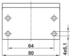
Angled bracket for the pillar, AISI 304, for gates with ascending hinges, part no. 205272
