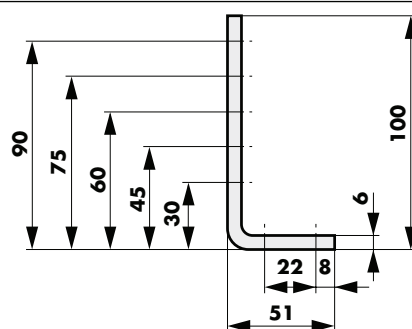
Mounting bracket for special applications part no. 205264 (zinc-plated) or 205267 (AISI 304)
