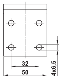
Angled bracket for the pillar, zinc-plated, for gates with ascending hinges, part no. 205452
